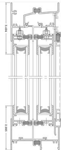
THERMAL BREAK ALUMINUM WINDOW SLIDER 2200 SERIES SIDE VIEW (1:1)
