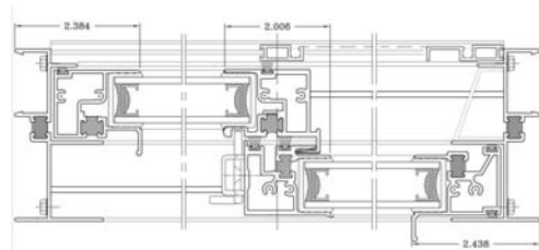
THERMAL BREAK ALUMINUM WINDOW SLIDER 2200 SERIES TOP VIEW (1:1)
