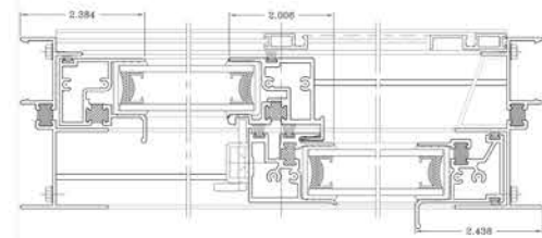
THERMAL BREAK ALUMINUM WINDOW SLIDER 2200 SERIES TOP VIEW (1:1)
